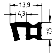
Art. 834551 RAU-SIK 8466 50±5° Shore A
