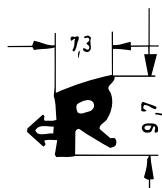
Art. 834101 RAU-SIK 8584 45±5° Shore A
