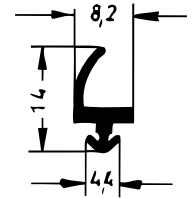
Art. 833291 RAU-SIK 8367 60±5° Shore A
