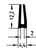
Art. 837200 RAU-SIK 8964 70±5° Shore A
