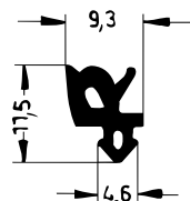
Art. 835481 RAU-SIK 8134 60±5° Shore A
