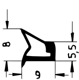
Art. 836870 RAU-SIK 8467 55±5° Shore A
