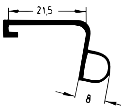
Art. 835220 RAU-SIK 8460 55±5° Shore A
