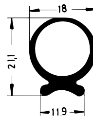
Art. 835520 RAU-SIK 8460 55±5° Shore A
