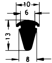
Art. 837240 RAU-SIK 8763 75±5° Shore A
