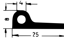
Art. 832700 RAU-SIK 8726 50±5° Shore A
