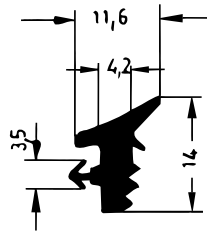
Art. 836890 RAU-SIK 8157 60±5° Shore A
