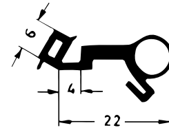
Art. 835640 RAU-SIK 8465 60±5° Shore A
