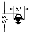
Art. 833131 RAU-SIK 8160 70±5° Shore A
