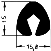
Art. 833531 RAU-SIK 8640 50±5° Shore A
