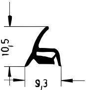
Art. 837880 RAU-SIK 8318 60±5° Shore A
