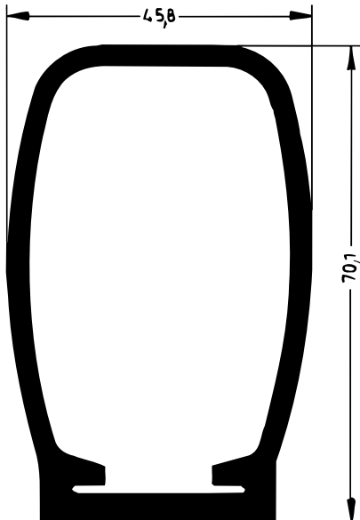
Art. 835501 RAU-SIK 8964 70±5° Shore A
