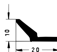
Art. 833951 RAU-SIK 8324 22±5° Shore A
