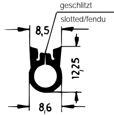
Art. 837060 RAU-SIK 8360 60±5° Shore A
