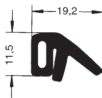
Art. 834532 RAU-SIK 8270 50±5° Shore A
