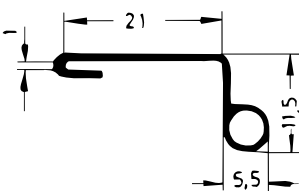
Art. 836000 RAU-SIK 8720 50±5° Shore A
