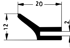
Art. 832721 RAU-SIK 8324 22±5° Shore A
