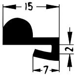
Art. 832660 RAU-SIK 8726 50±5° Shore A
