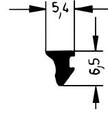
Art. 834321 RAU-SIK 8760 70±5° Shore A
