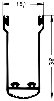
Art. 837760 RAU-SIK 8360 60±5° Shore A
