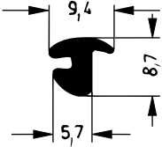
Art. 833761 RAU-SIK 8220 55±5° Shore A
