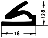
Art. 833891 RAU-SIK 8270 50±5° Shore A
