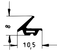
Art. 834151 RAU-SIK 8367 60±5° Shore A
