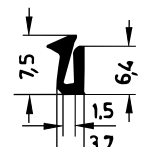
Art. 835700 RAU-SIK 8163 70±5° Shore A
