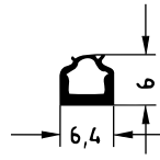
Art. 834761 RAU-SIK 8968 50±5° Shore A
