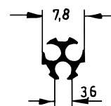
Art. 837720 RAU-SIK 8130 60±5° Shore A
