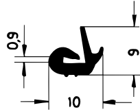
Art. 836310 RAU-SIK 8318 60±5° Shore A
