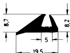
Art. 836580 RAU-SIK 8367 60±5° Shore A
