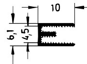
Art. 837510 RAU-SIK 8110 40±5° Shore A
