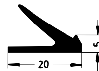
Art. 834590 RAU-SIK 8460 55±5° Shore A
