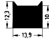
Art. 832540 RAU-SIK 8726 50±5° Shore A
