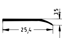
Art. 832841 RAU-SIK 8960 65±5° Shore A
