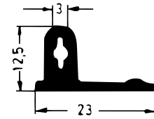
Art. 833410 RAU-SIK 8726 50±5° Shore A
