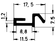
Art. 833610 RAU-SIK 8726 50±5° Shore A
