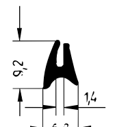
Art. 837870 RAU-SIK 8128 55±5° Shore A
