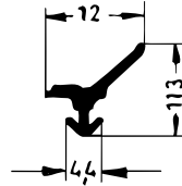
Art. 835570 RAU-SIK 8360 60±5° Shore A
