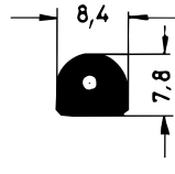
Art. 836730 RAU-SIK 8160 70±5° Shore A
