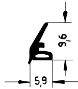
Art. 837990 RAU-SIK 8318 60±5° Shore A
