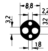
Art. 836930 RAU-SIK 8360 60±5° Shore A
