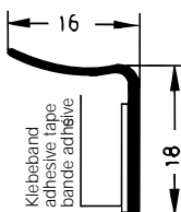
Art. 837620 RAU-SIK 8960 65±5° Shore A
