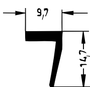
Art. 835701 RAU-SIK 8855 70±5° Shore A
