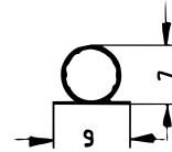
Art. 834262 RAU-SIK 8760 70±5° Shore A
