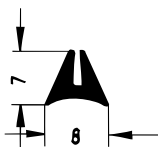
Art. 834191 RAU-SIK 8367 60±5° Shore A
