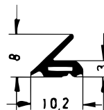
Art. 833191 RAU-SIK 8466 50±5° Shore A
