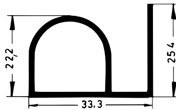
Art. 836670 RAU-SIK 8367 60±5° Shore A
