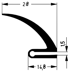
Art. 837430 RAU-SIK 8760 70±5° Shore A
