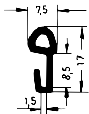
Art. 833650 RAU-SIK 8726 50±5° Shore A
