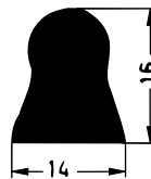
Art. 832680 RAU-SIK 8134 60±5° Shore A
