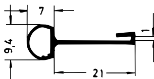
Art. 835920 RAU-SIK 8460 55±5° Shore A
