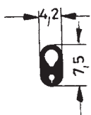
Art. 834273 RAU-SIK 8130 60±5° Shore A
