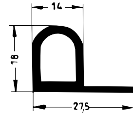
Art. 835551 RAU-SIK 8367 60±5° Shore A
