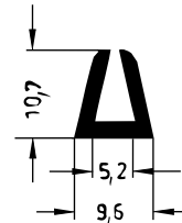
Art. 835741 RAU-SIK 8128 55±5° Shore A
