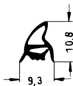
Art. 833081 RAU-SIK 8318 60±5° Shore A
