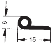
Art. 834383 RAU-SIK 8505 66±5° Shore A
