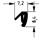
Art. 834081 RAU-SIK 8961 70±5° Shore A
