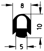
Art. 835030 RAU-SIK 8940 60±5° Shore A
