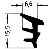
Art. 836900 RAU-SIK 8587 70±5° Shore A
