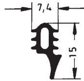
Art. 834133 RAU-SIK 8317 65±5° Shore A
