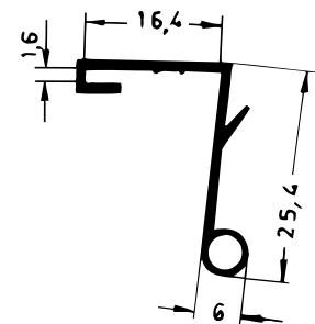
Art. 836290 RAU-SIK 8367 60±5° Shore A
