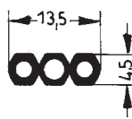
Art. 834962 RAU-SIK 9600 60±5° Shore A
