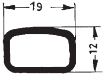
Art. 833500 RAU-SIK 8230 50±5° Shore A
