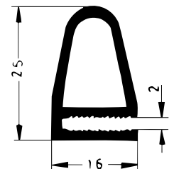
Art. 833501 RAU-SIK 8367 60±5° Shore A
