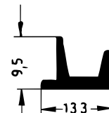
Art. 833791 RAU-SIK 8180 80±5° Shore A
