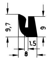
Art. 832820 RAU-SIK 8726 50±5° Shore A
