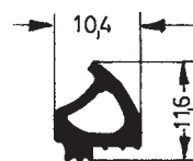
Art. 834862 RAU-SIK 8119 40±5° Shore A
