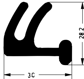
Art. 832391 RAU-SIK 8253 65±5° Shore A
