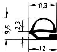
Art. 835990 RAU-SIK 8460 55±5° Shore A
