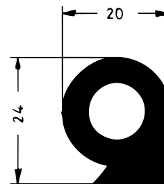
Art. 832601 RAU-SIK 8640 50±5° Shore A
