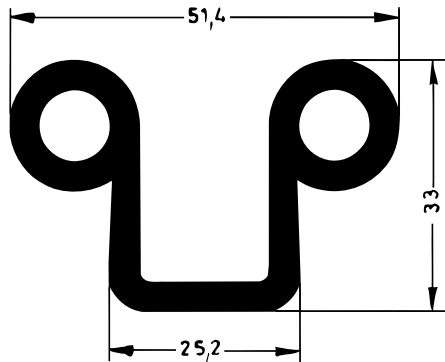
Art. 835641 RAU-SIK 8367 60±5° Shore A
