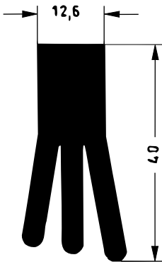
Art. 834382 RAU-SIK 8270 50±5° Shore A
