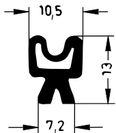
Art. 835691 RAU-SIK 8640 50±5° Shore A
