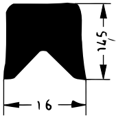
Art. 833101 RAU-SIK 8361 60±5° Shore A
