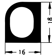
Art. 837170 RAU-SIK 8110 40±5° Shore A
