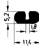
Art. 832131 RAU-SIK 8270 50±5° Shore A
