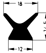
Art. 835980 RAU-SIK 8284 28±5° Shore A
