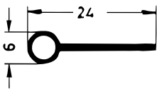
Art. 835010 RAU-SIK 8460 55±5° Shore A
