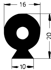
Art. 832321 RAU-SIK 8640 50±5° Shore A
