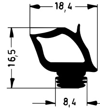
Art. 833121 RAU-SIK 8110 40±5° Shore A
