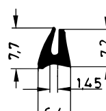
Art. 836250 RAU-SIK 8460 55±5° Shore A
