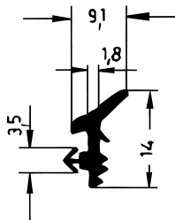
Art. 836880 RAU-SIK 8157 60±5° Shore A
