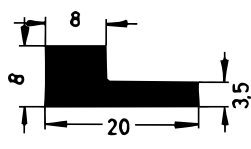
Art. 833760 RAU-SIK 8280 33±5° Shore A
