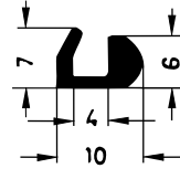
Art. 833340 RAU-SIK 8280 33±5° Shore A
