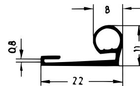
Art. 836570 RAU-SIK 8740 60±5° Shore A
