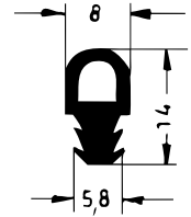
Art. 834511 RAU-SIK 8324 22±5° Shore A
