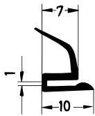
Art. 833770 RAU-SIK 8726 50±5° Shore A
