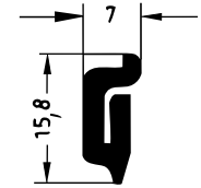
Art. 833251 RAU-SIK 8110 40±5° Shore A
