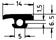
Art. 835050 RAU-SIK 8910 50±5° Shore A
