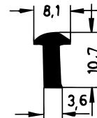
Art. 835630 RAU-SIK 8128 55° Shore A
