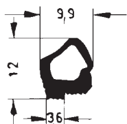
Art. 834721 RAU-SIK 8110 40±5° Shore A
