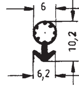
Art. 834102 RAU-SIK 8163 70±5° Shore A
