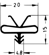
Art. 832361 RAU-SIK 8168 70±5° Shore A
