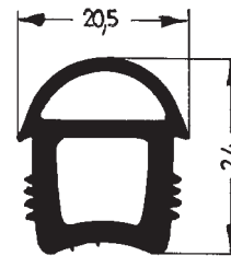
Art. 834882 RAU-SIK 8128 55±5° Shore A
