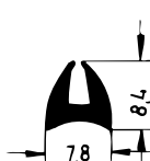
Art. 834521 RAU-SIK 8270 50±5° Shore A
