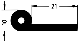
Art. 833450 RAU-SIK 8726 50±5° Shore A
