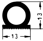
Art. 834471 RAU-SIK 8360 60±5° Shore A
