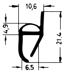
Art. 835850 RAU-SIK 8726 50±5° Shore A
