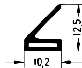
Art. 837830 RAU-SIK 8318 60±5° Shore A
