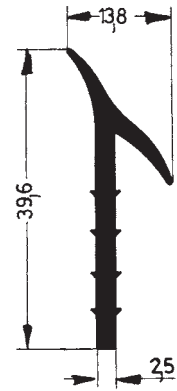
Art. 834393 RAU-SIK 8976 65±5° Shore A
