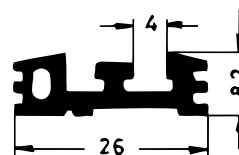
Art. 835040 RAU-SIK 8460 55±5° Shore A
