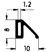
Art. 835070 RAU-SIK 8467 55±5° Shore A
