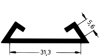
Art. 832251 RAU-SIK 8318 65±5° Shore A
