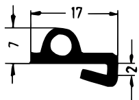
Art. 832880 RAU-SIK 8726 50±5° Shore A
