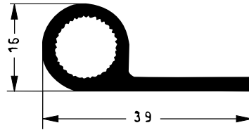
Art. 833061 RAU-SIK 8270 50±5° Shore A
