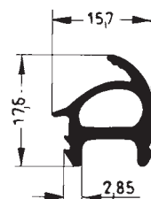
Art. 835861 RAU-SIK 8460 55±5° Shore A
