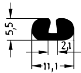
Art. 835490 RAU-SIK 8931 60±5° Shore A
