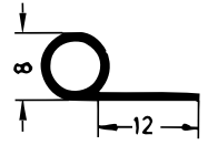
Art. 833600 RAU-SIK 8726 50±5° Shore A
