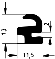
Art. 837920 RAU-SIK 8110 40±5° Shore A
