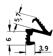
Art. 836780 RAU-SIK 8760 70±5° Shore A
