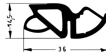
Art. 835661 RAU-SIK 8273 70±5° Shore A
