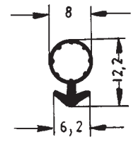
Art. 834092 RAU-SIK 8163 70±5° Shore A
