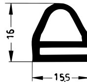
Art. 835561 RAU-SIK 8110 40±5° Shore A
