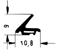
Art. 834731 RAU-SIK 8466 50±5° Shore A
