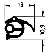
Art. 836530 RAU-SIK 8466 50±5° Shore A
