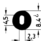
Art. 832670 RAU-SIK 8726 50±5° Shore A
