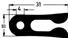
Art. 832310 RAU-SIK 8128 55±5° Shore A
