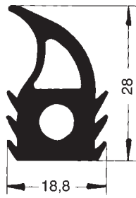
Art. 834531 Z RAU-SIK 8270 50±5° Shore A
