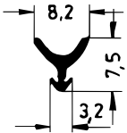
Art. 835080 RAU-SIK 8360 60±5° Shore A
