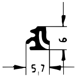
Art. 833681 RAU-SIK 8355 25±5° Shore A
