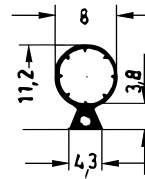
Art. 833721 RAU-SIK 8167 70±5° Shore A
