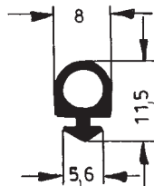
Art. 834562 RAU-SIK 8270 50±5° Shore A
