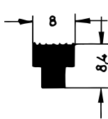
Art. 836240 RAU-SIK 8760 70±5° Shore A
