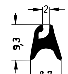
Art. 835940 RAU-SIK 8460 55±5° Shore A
