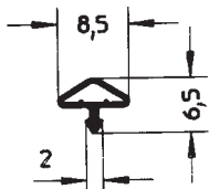
Art. 834972 RAU-SIK 8220 55±5° Shore A
