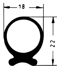
Art. 833621 RAU-SIK 8190 55±5° Shore A
