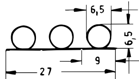
Art. 837790 RAU-SIK 8158 60±5° Shore A
