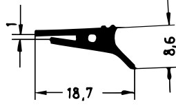
Art. 835500 RAU-SIK 8943 60±5° Shore A
