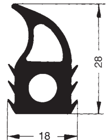
Art. 835711 RAU-SIK 8806 50±5° Shore A
