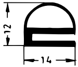
Art. 833851 RAU-SIK 8360 60±5° Shore A
