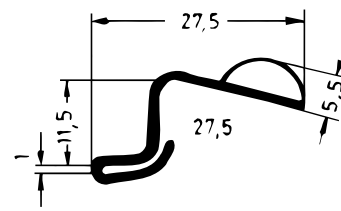
Art. 836050 RAU-SIK 8318 60±5° Shore A
