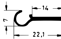
Art. 835600 RAU-SIK 8460 55±5° Shore A
