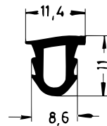
Art. 836860 RAU-SIK 8855 70±5° Shore A
