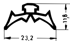
Art. 833811 RAU-SIK 8360 60±5° Shore A
