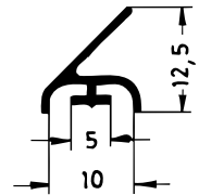
Art. 835110 RAU-SIK 8367 60±5° Shore A
