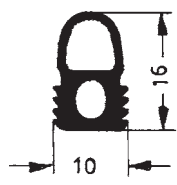
Art. 834912 RAU-SIK 8270 50±5° Shore A
