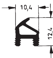
Art. 834762 Z RAU-SIK 8153 60±5° Shore A
