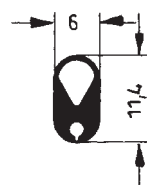
Art. 834922 RAU-SIK 8130 60±5° Shore A
