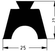
Art. 832641 RAU-SIK 8640 50±5° Shore A
