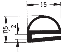
Art. 833853 RAU-SIK 8270 50±5° Shore A
