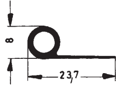
Art. 835111 RAU-SIK 8467 55±5° Shore A
