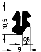
Art. 836070 RAU-SIK 8110 40±5° Shore A
