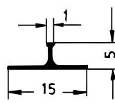
Art. 835330 RAU-SIK 8463 50±5° Shore A
