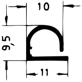
Art. 835930 RAU-SIK 8460 55±5° Shore A
