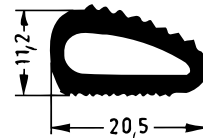
Art. 834221 RAU-SIK 8128 55±5° Shore A
