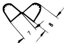
Art. 834591 RAU-SIK 8158 60±5° Shore A
