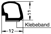
Art. 834111 RAU-SIK 8586 65±5° Shore A
