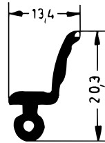
Art. 834001 RAU-SIK 8367 60±5° Shore A
