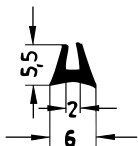
Art. 836770 RAU-SIK 8360 60±5° Shore A
