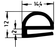
Art. 837280 RAU-SIK 8128 55±5° Shore A
