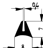
Art. 835591 RAU-SIK 8367 60±5° Shore A
