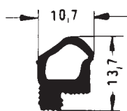
Art. 834711 RAU-SIK 8110 40±5° Shore A
