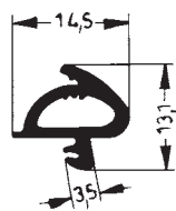
Art. 835841 RAU-SIK 8466 50±5° Shore A
