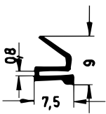
Art. 834710 RAU-SIK 8460 55±5° Shore A
