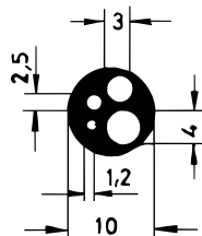
Art. 836120 RAU-SIK 8123 50±5° Shore A
