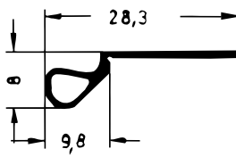
Art. 835540 RAU-SIK 8465 60±5° Shore A
