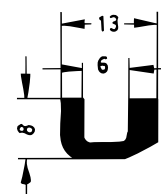
Art. 836630 RAU-SIK 8128 55±5° Shore A
